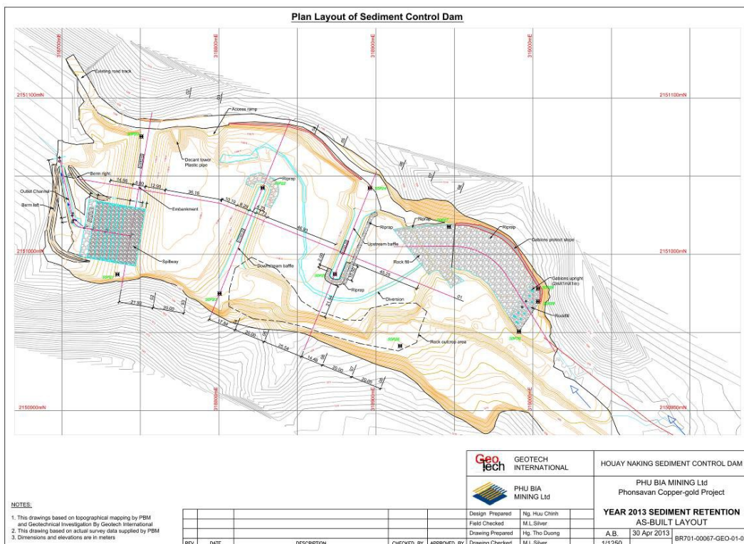
Plan view of layout of the Houay Naking Sediment Management Dam and Sediment Retention Pond – Lao PDR
